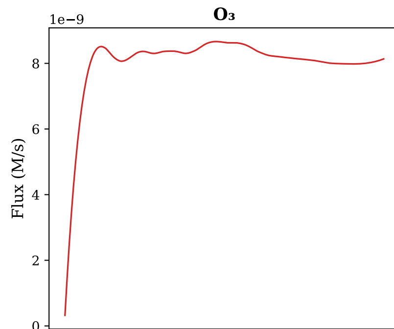
Mass transfer flux by BC type (DIW, 600 s)
